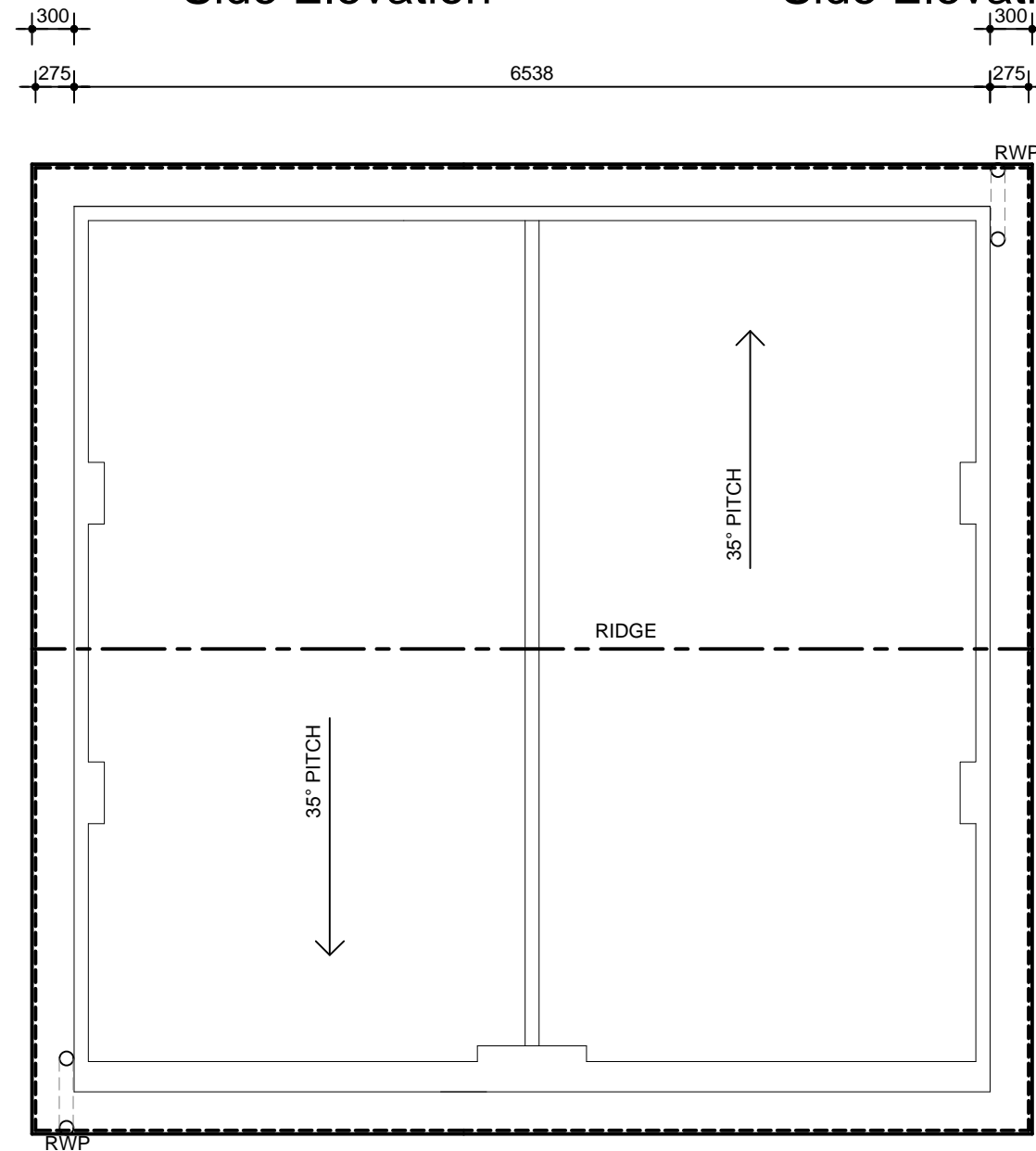
Roof Plan
