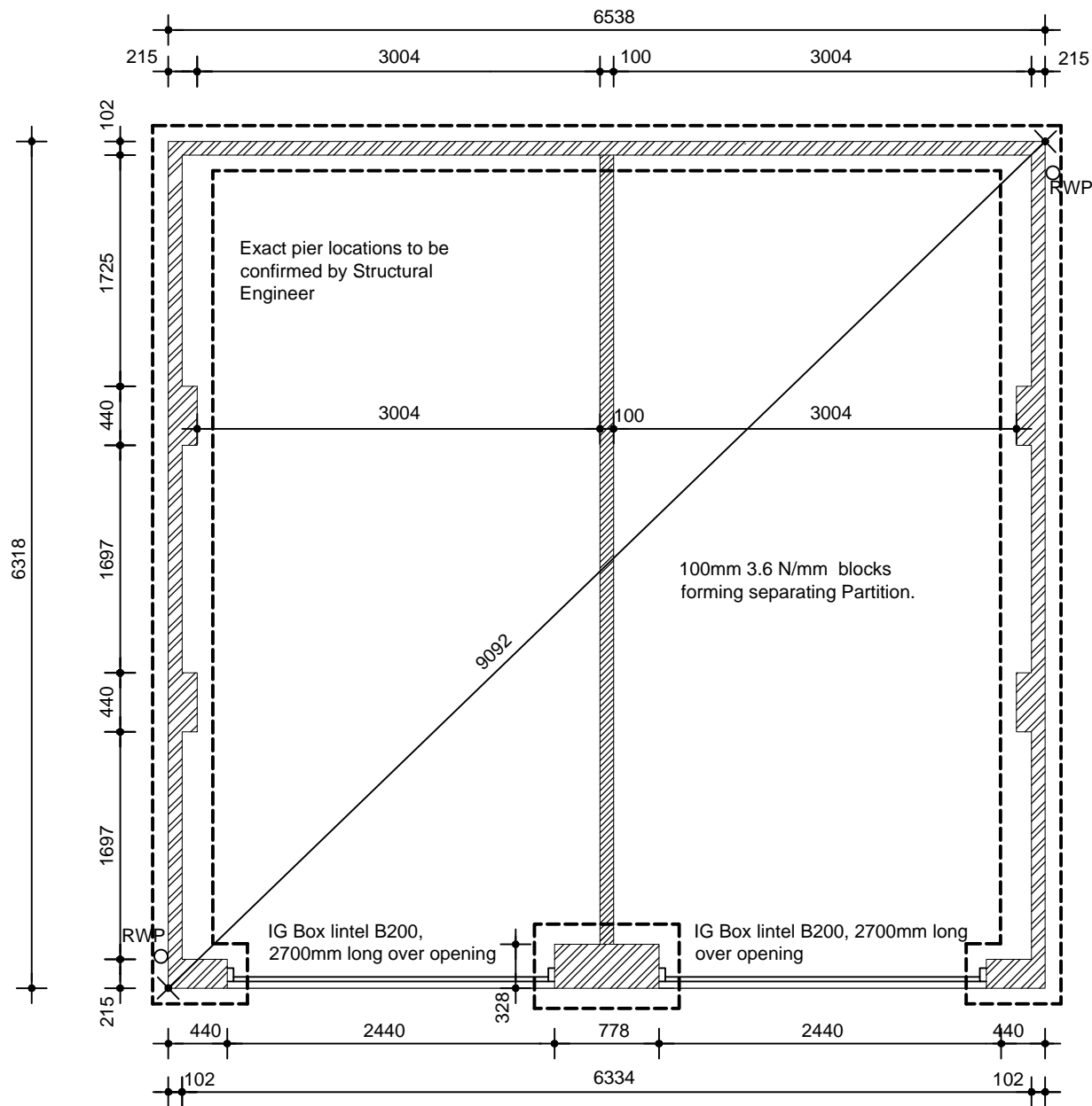
Floor Plan
