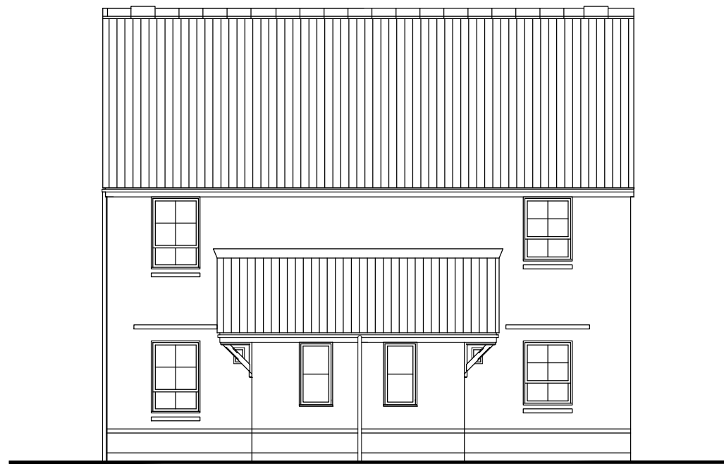
FRONT ELEVATION
