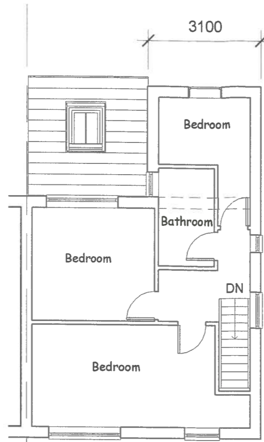
2 First Floor 1 : 100
