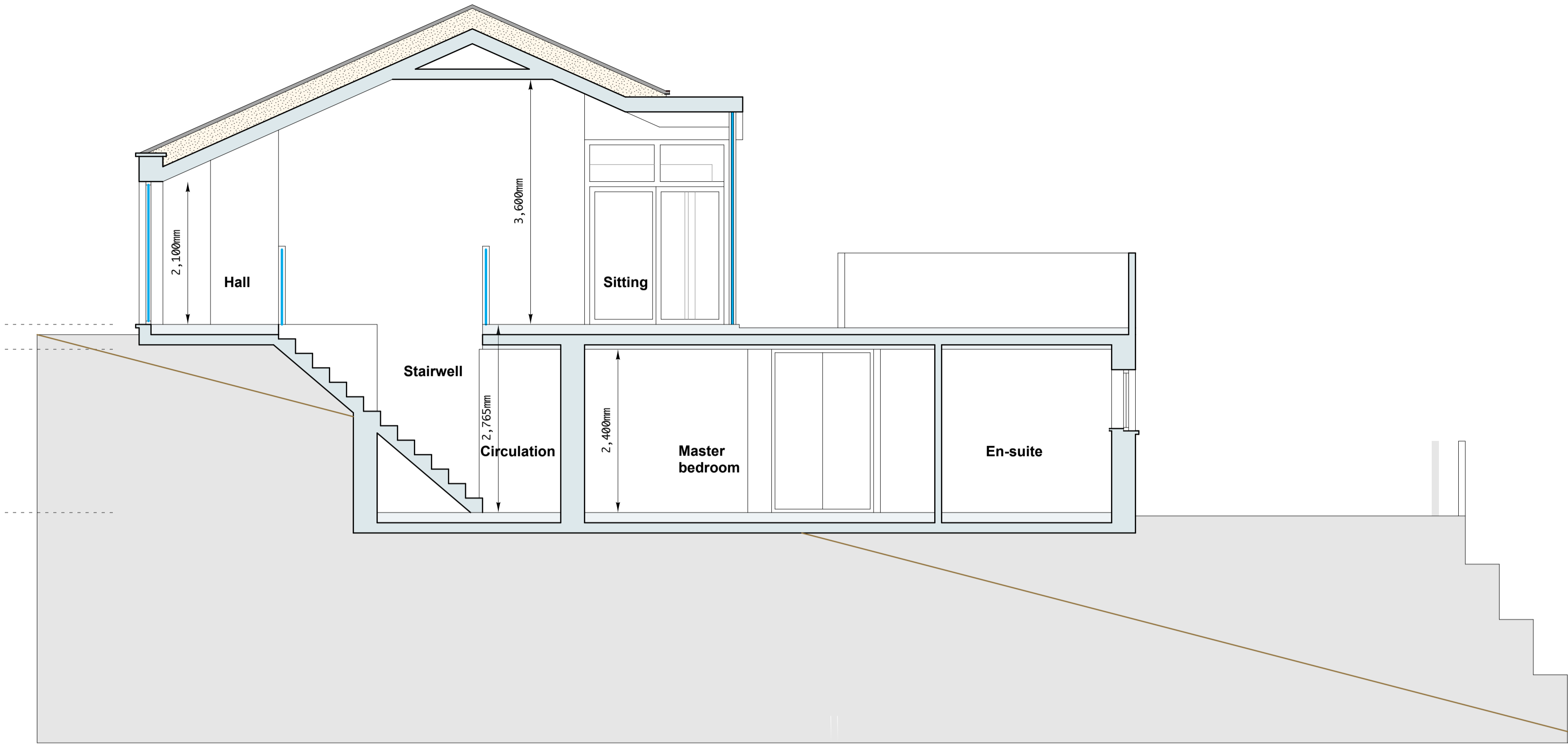
SECTION - EE
