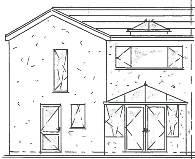
REAR ELEVATIONS PROPOSED
