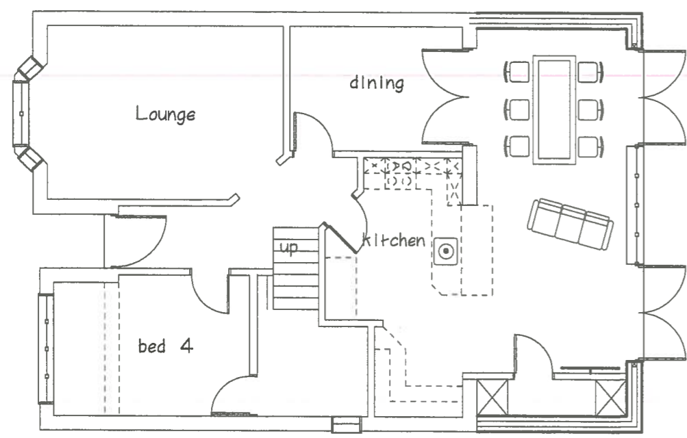
Proposed plan on ground floor
