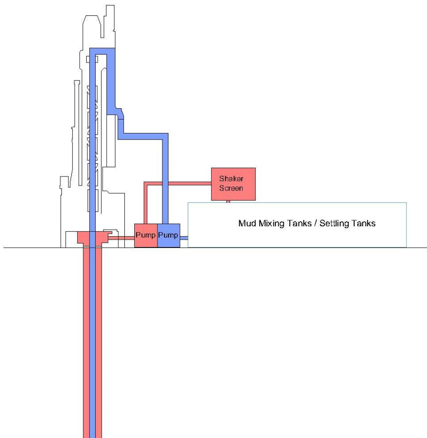
Figure 2: Close Loop System for the drilling fluids
