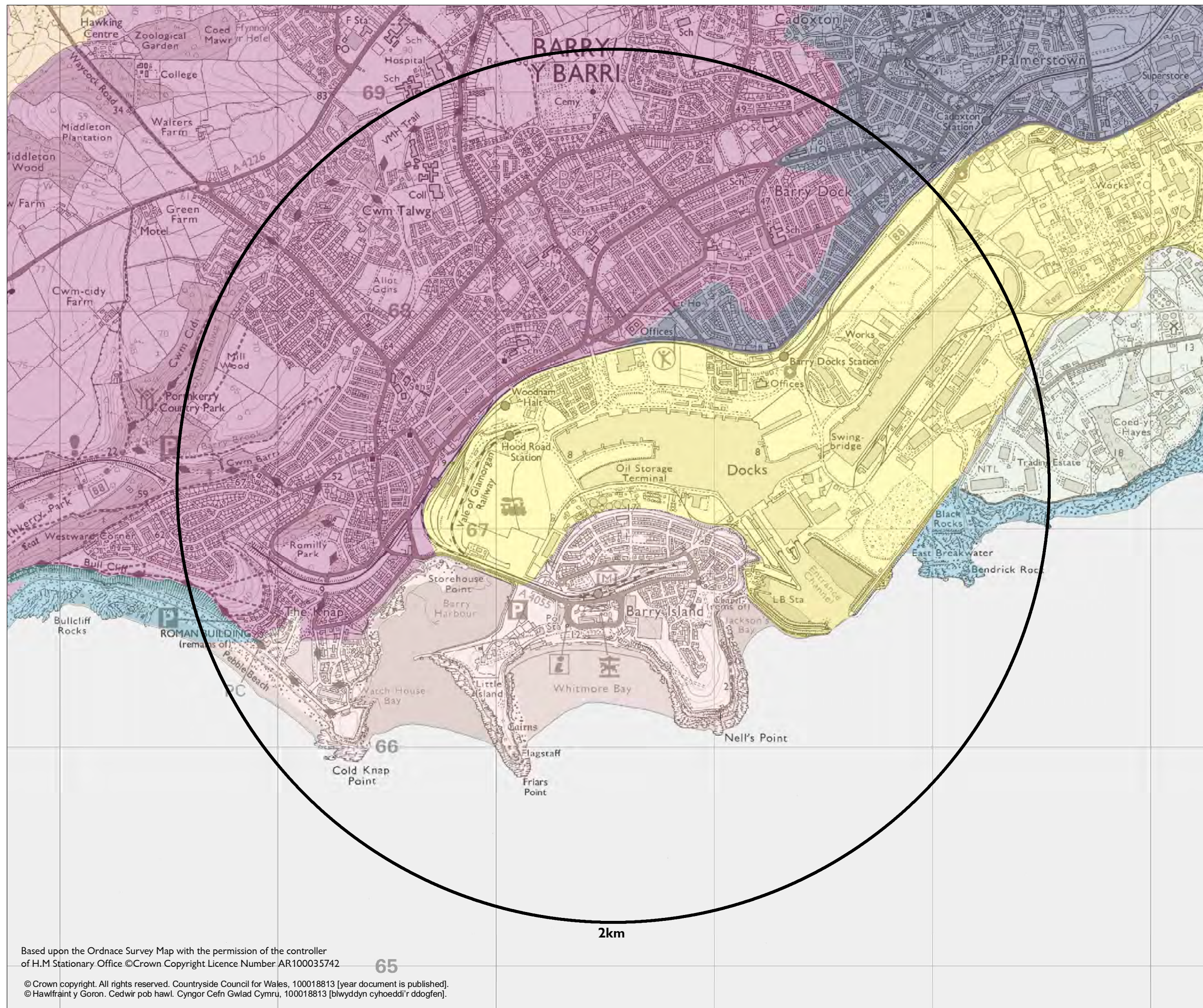
FIGURE E9: LANDMAP DATA GEOLOGICAL LANDSCAPE (LEVEL 3 CLASSIFICATION)
