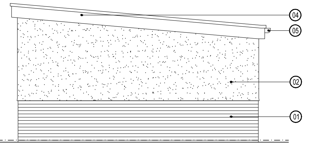
CYCLE STORE SIDE ELEVATION
