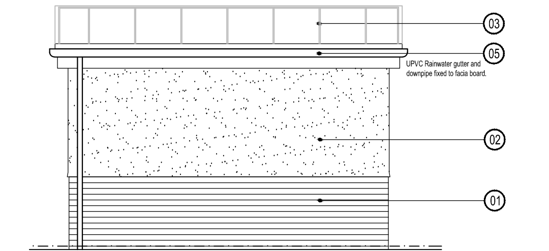
CYCLE STORE REAR ELEVATION
