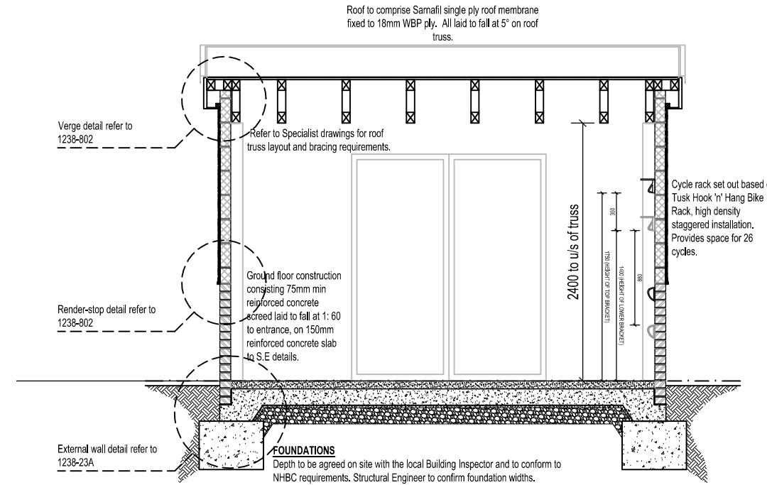
CYCLE STORE SECTION A-A
