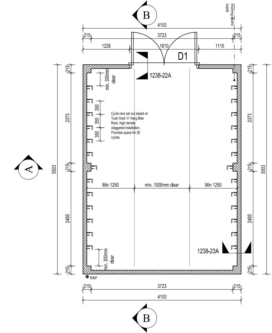
CYCLE STORE GROUND FLOOR PLAN
