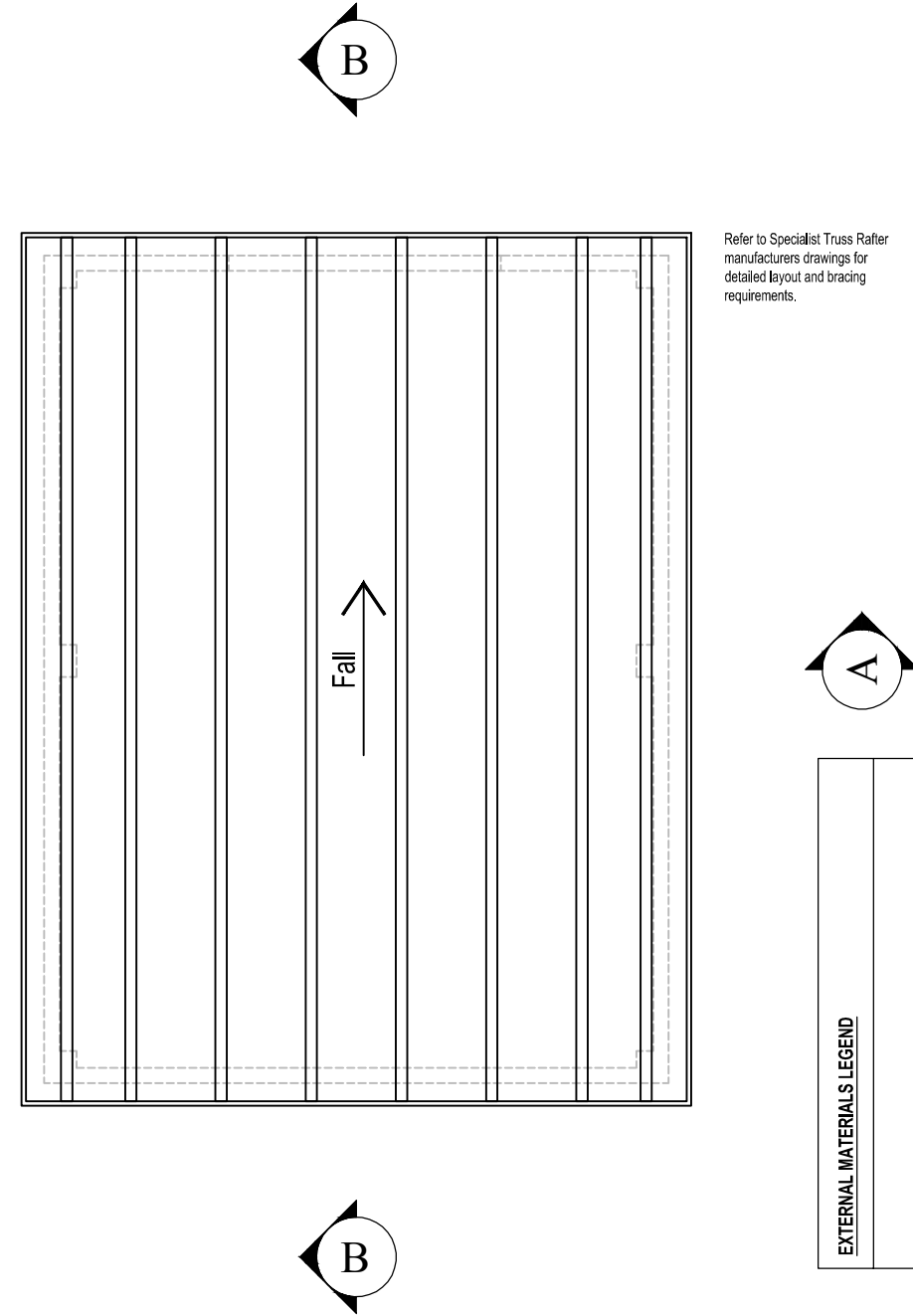
CYCLE STORE ROOF PLAN
