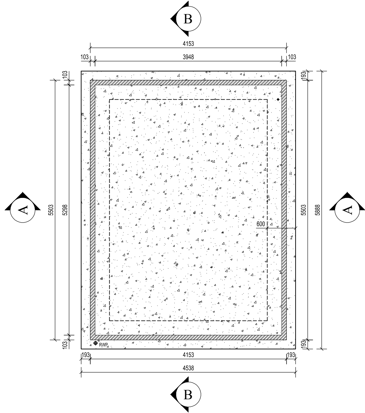
CYCLE STORE FOUNDATION PLAN
