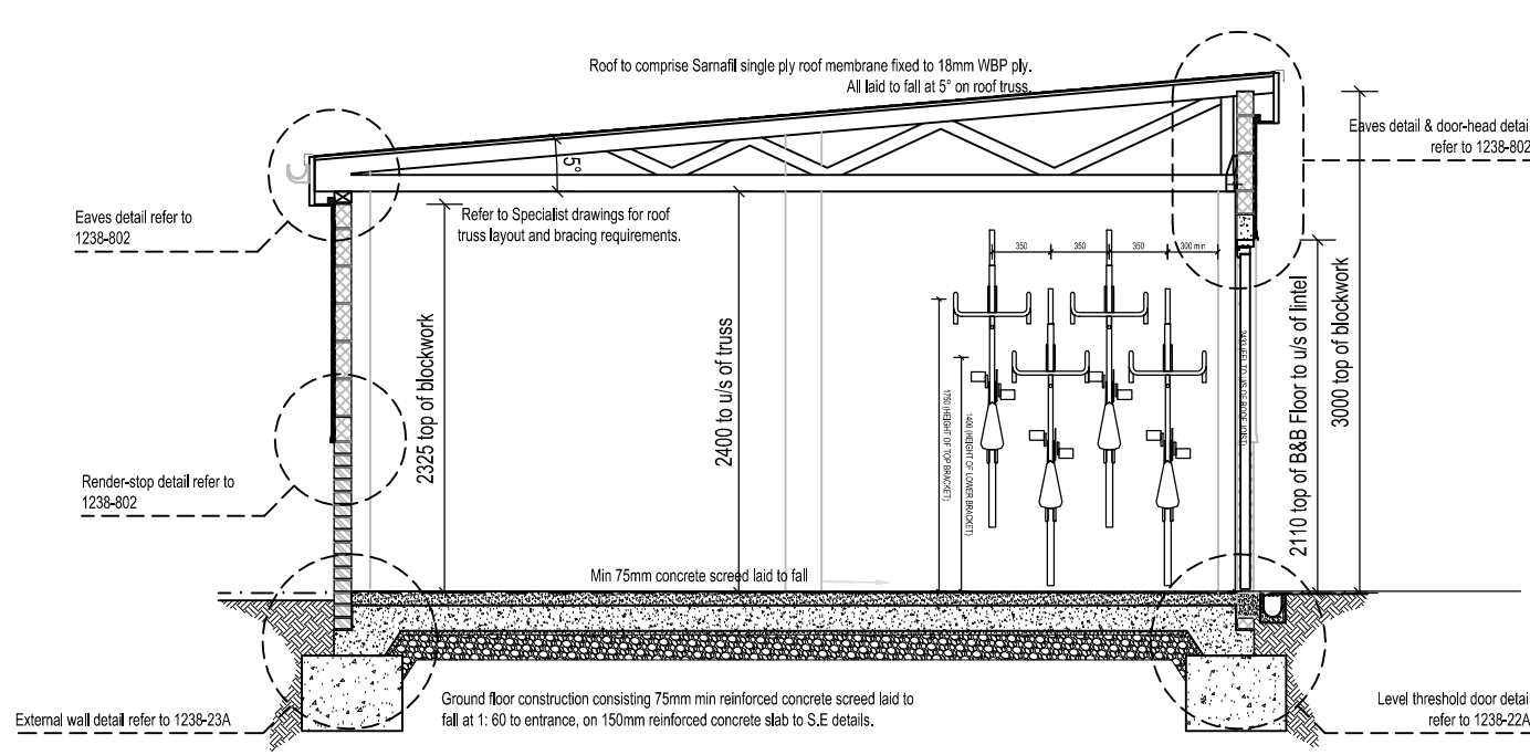
CYCLE STORE SECTION B-B
