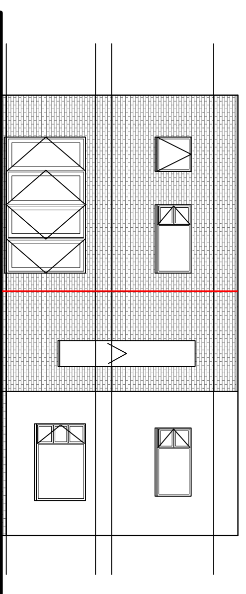
Rear Elevation - 1:100
