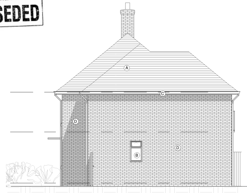
East (Side) Elevation 1 : 100
