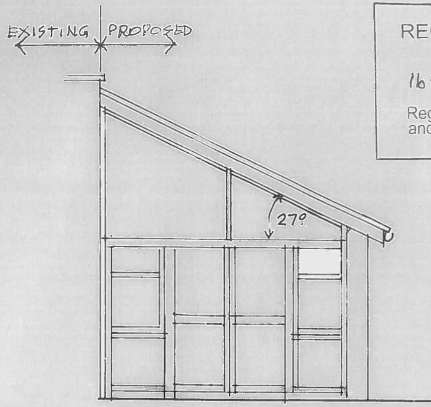
SOUTH-EAST ELEVATION
