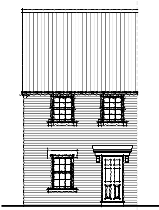
Front Elevation
