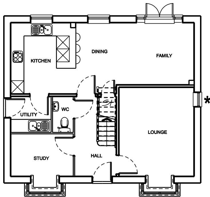
GROUND FLOOR PLANS
